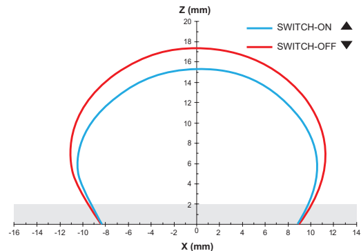
Typical switch-on and switch-off sensing distances along X axis as function of Z.
