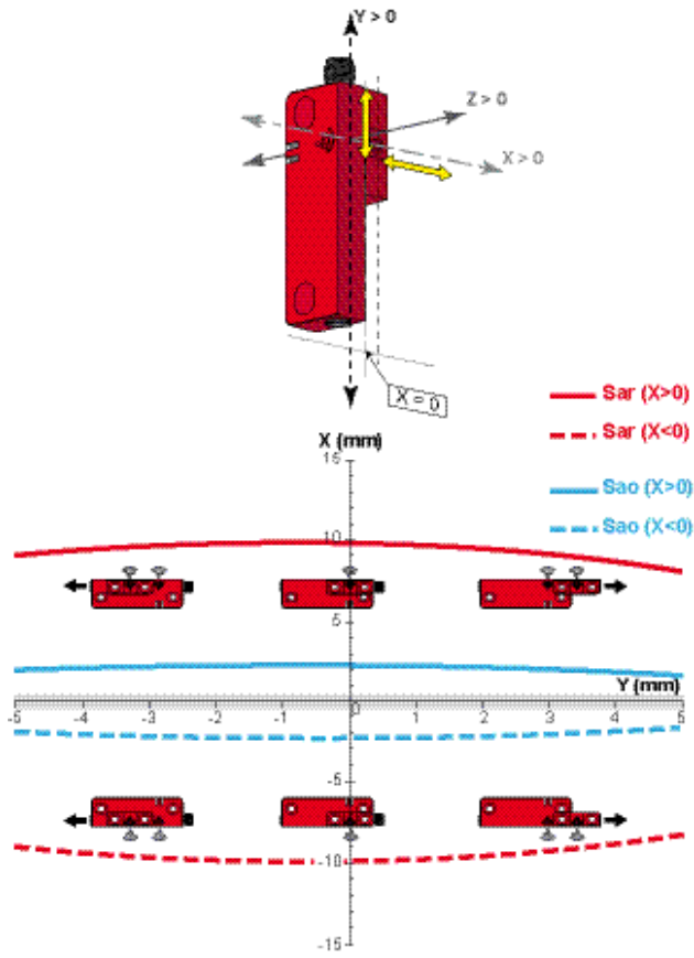
Figure of S_{ao} and S_{ar} sensing distances along Y axis as function of X
