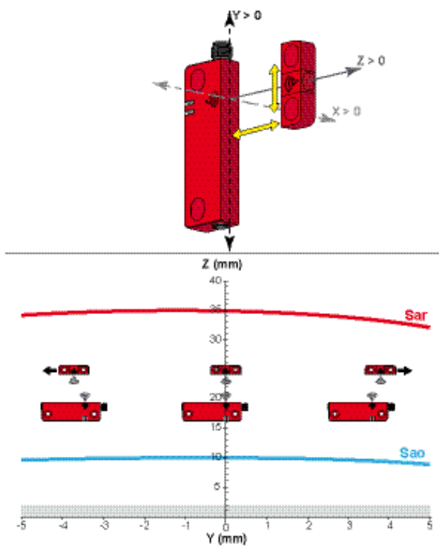
Typical switch-on and switch-off sensing distances along Y axis as function of Z.
