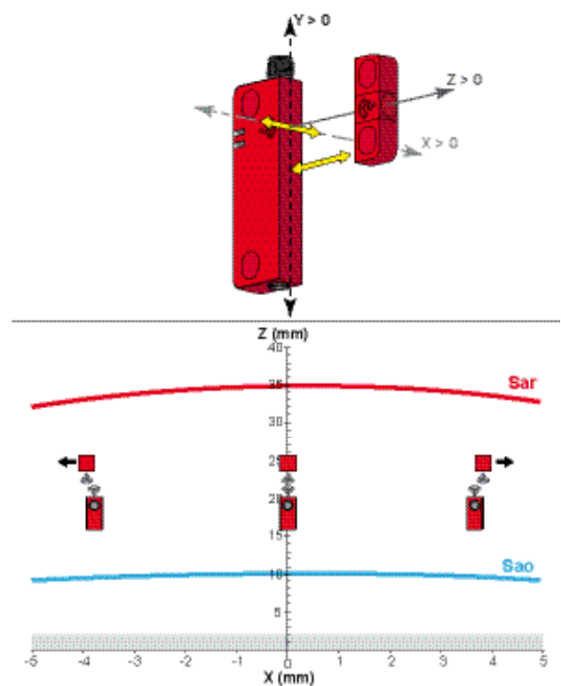
Typical switch-on and switch-off sensing distances along X axis as function of Z.
