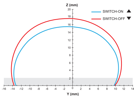
Typical switch-on and switch-off sensing distances along Y axis as function of Z.
