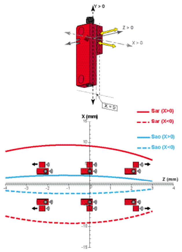
Figure of S_{ao} and S_{ar} sensing distances along Z axis as function of X
