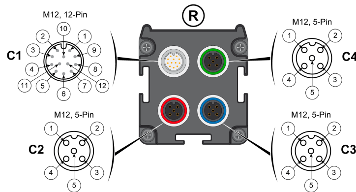
C1 - GRAY CONNECTOR - Main male connector (M12, 12-Pin):
