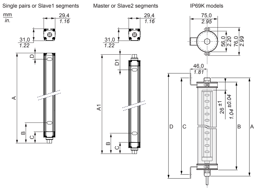
Single Pair or Secondary Segment 1 Dimensions (in mm)
